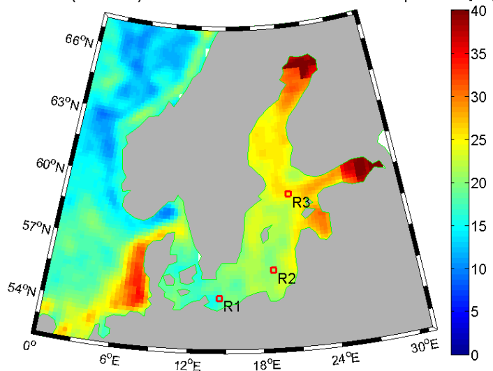
AVISO (satellite) Sea Level Anomalies Data - Amplitude [cm]
