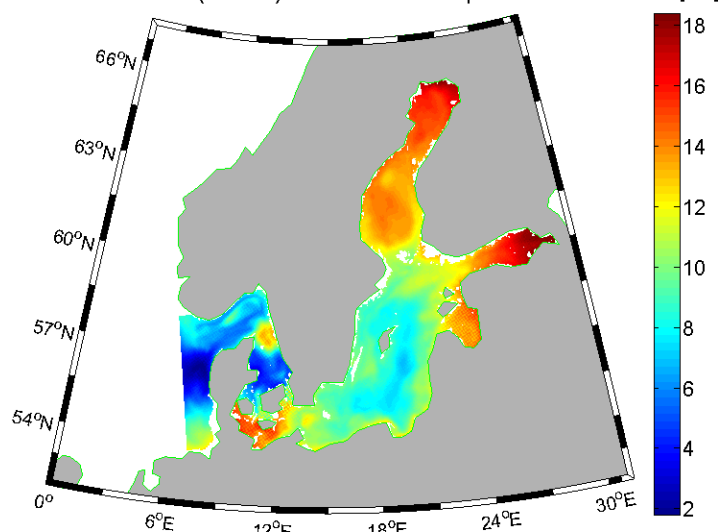
POP (model) SLA Data - Amplitude
